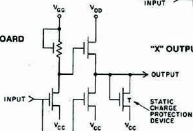
OUTPUT DRIVER
