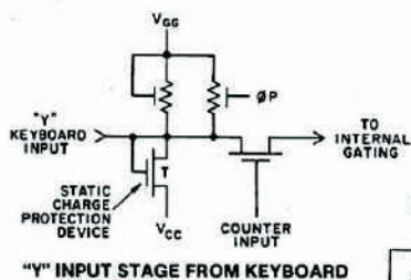
"Y" INPUT STAGE FROM KEYBOARD
