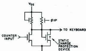
"X" OUTPUT STAGE TO KEYBOARD
