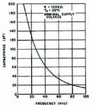
Fig.5 OSCILLATOR FREQUENCY vs. C_2
